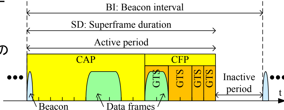
(a) Superframe in IEEE 802.15.4 MAC
